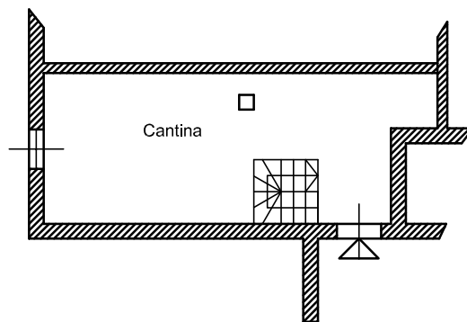
PIANO INTERRATO
